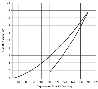
Fig. 1. Chart of loading distribution
